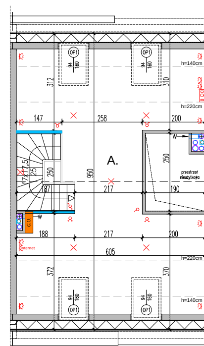
ANTRESOLA
